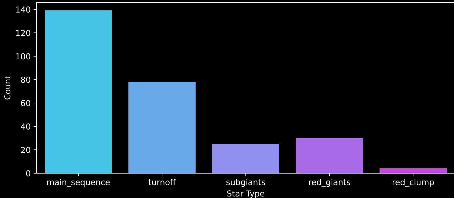
GALAH DR4 Field: [332] Count plot of Star Type
