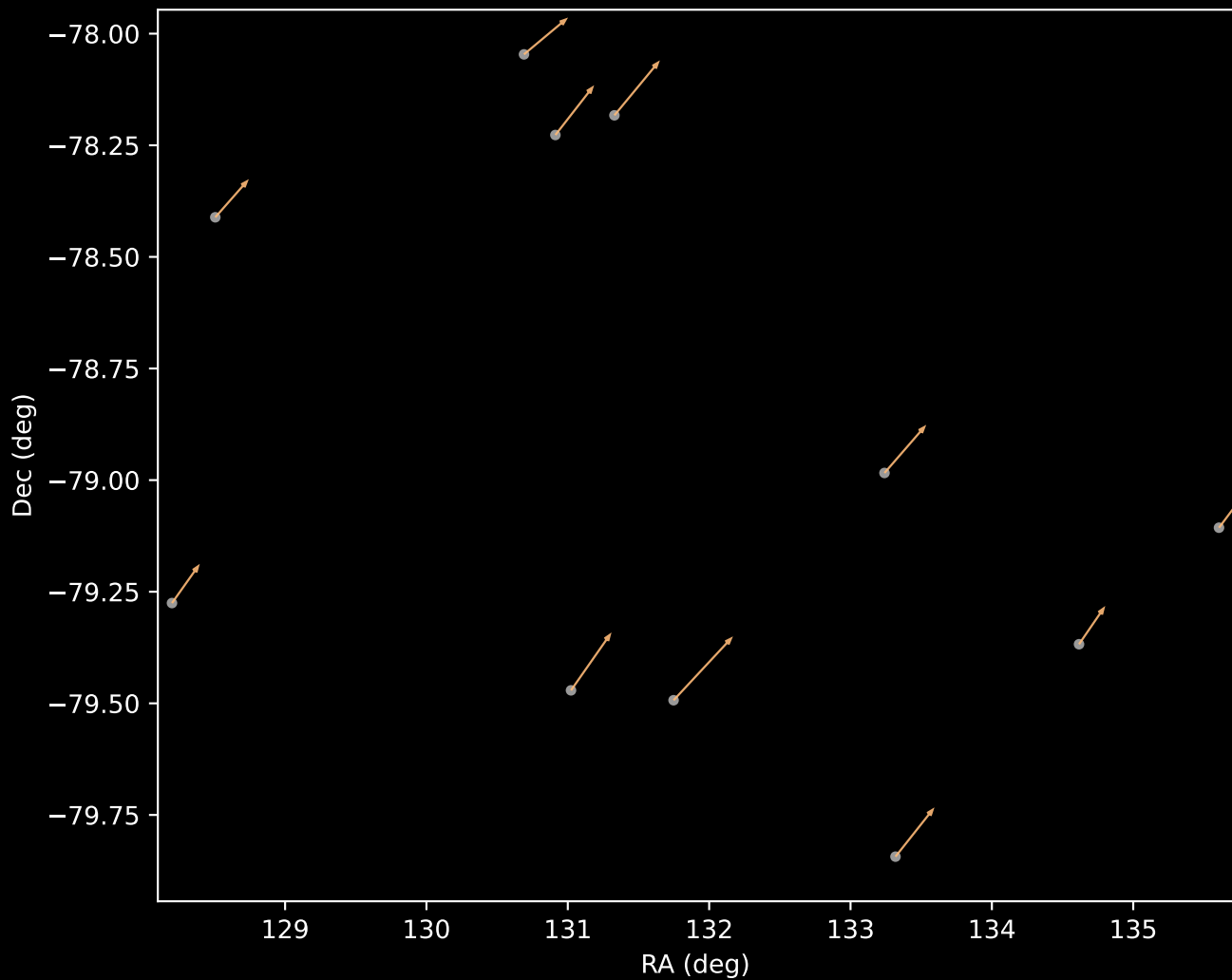
GALAH DR4 Cluster 3 Proper Motion Vectors (n=11)
