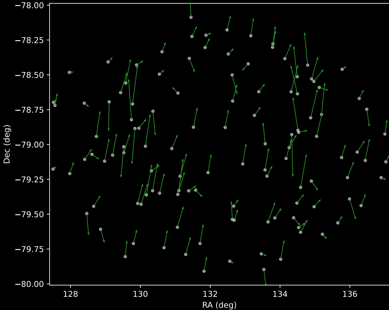
GALAH DR4 Cluster 4 Proper Motion Vectors (n=117)
